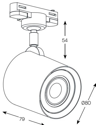
1 Ph Track 3242, 3243, 4244
